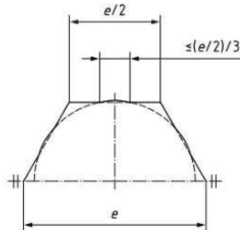
Figure 3 — Detail: Broached socket
