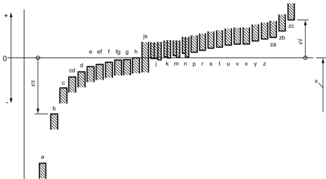
b) Shafts (external features of size)
