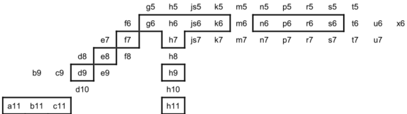
Figure 11 — Shafts
