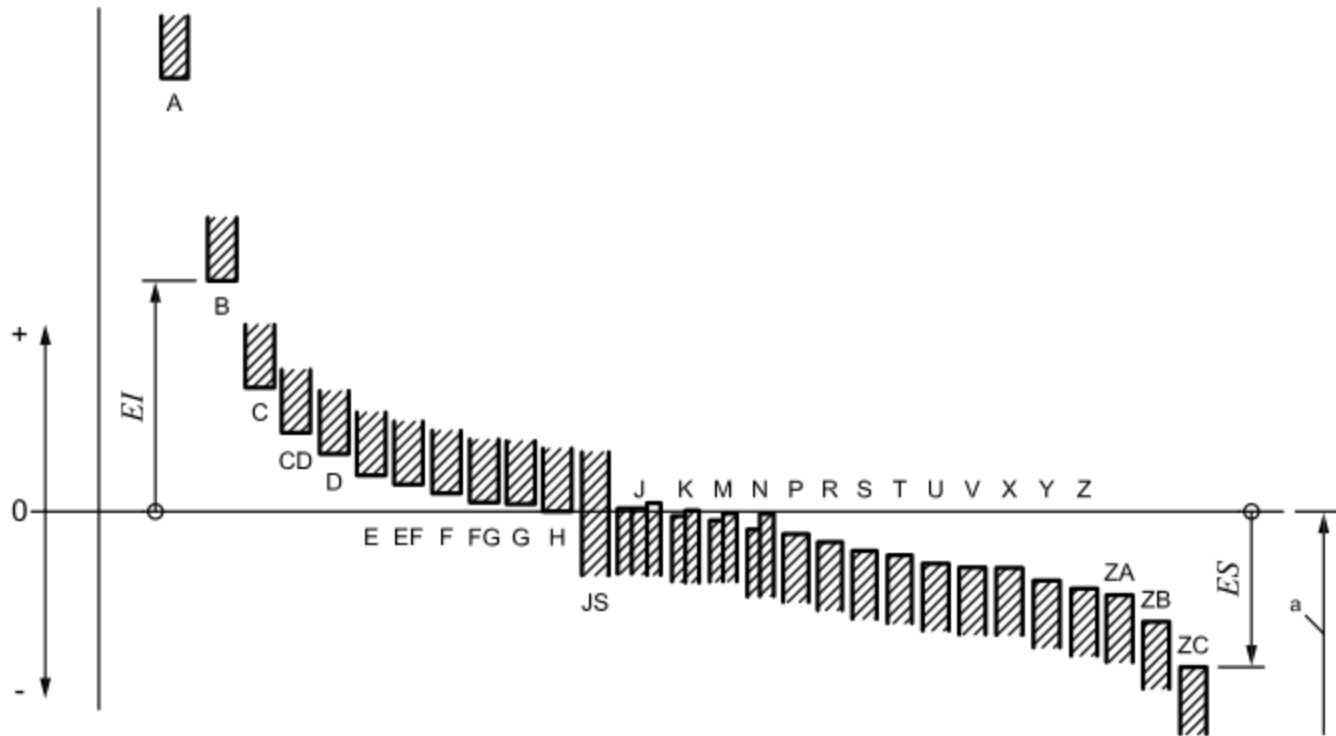
a) Holes (internal features of size)
