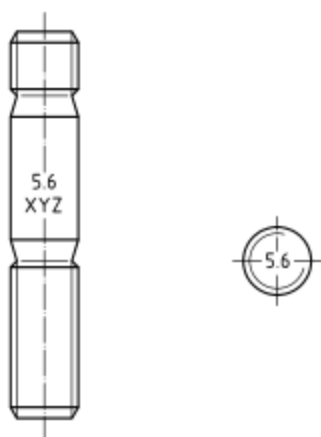
Figure 14 — Example of marking of studs
