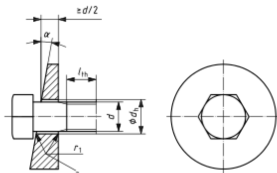
Figure 1 — Wedge loading of finished bolts and screws
