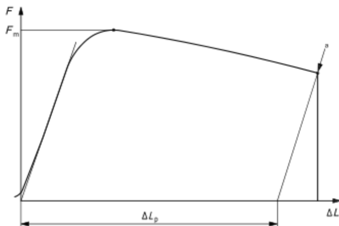
Figure 3 — Load-displacement curve for determination of elongation after fracture, A_t
