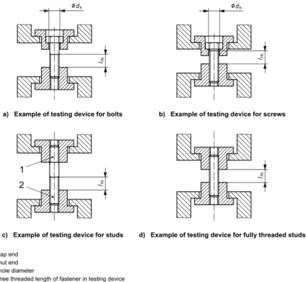
Figure 2 — Examples of testing devices
